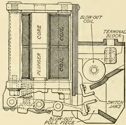
Fig. 60 Sprague-General Electric Contactor Diagram
